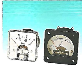
TH-38 Model: TH-38 Size: 44×44×35mm Panel cut-out Ø : 38mm
