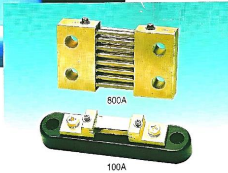
SHUNT 800A Model: Shunt 100A Range: 10-5000A F.S.: 50mv
