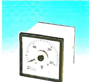
L-96 Model: L-96 Size: 96×96×110mm Panel cut-out □ : 90×90mm
