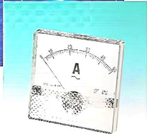
YS-10 Model: YS-10 Size: 100×100×50mm Panel cut-out Ø : 84mm
