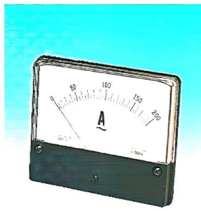
L-72 Model: L-72 Size: 72×72×85mm Panel cut-out □ : 66×66mm
