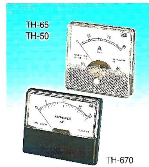
TH-65 Model: TH-65 Size: 66×66×40mm Panel cut-out □ : 52mm
