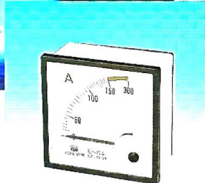
SR-96 Model: SR-96 Size: 96×96×65mm Panel cut-out □ : 90×90mm
