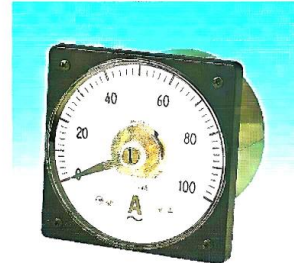
L-110 Model: L-110 Size: 110×110×95mm Panel cut-out □ : 102mm
